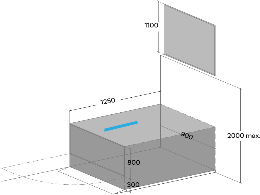
Figure 4.19 Platform lift
