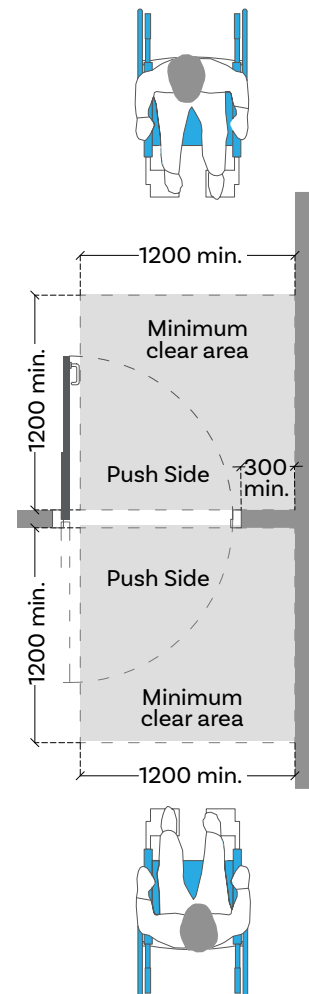
Fig c: Case of both-side push swinging doors
