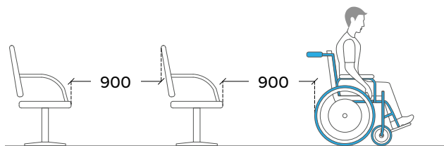
Fig c. Section
