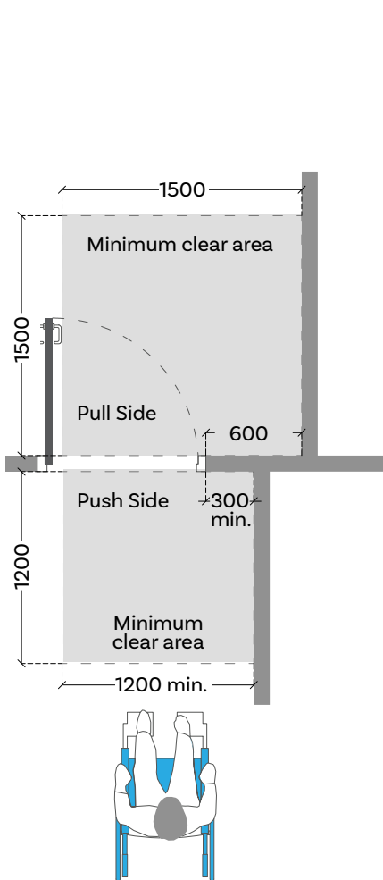
Fig a: Case of one push side swinging doors
