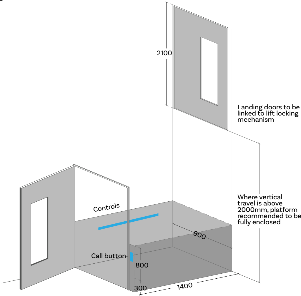
Figure 4.19 Platform lift
