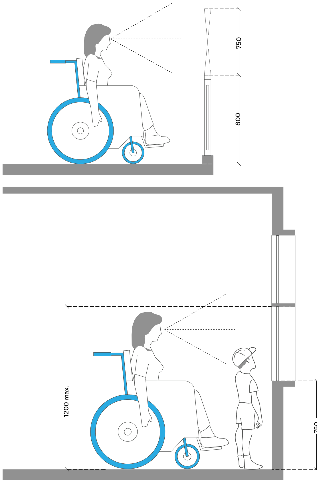
Figure 4.45 Unobstructed view
