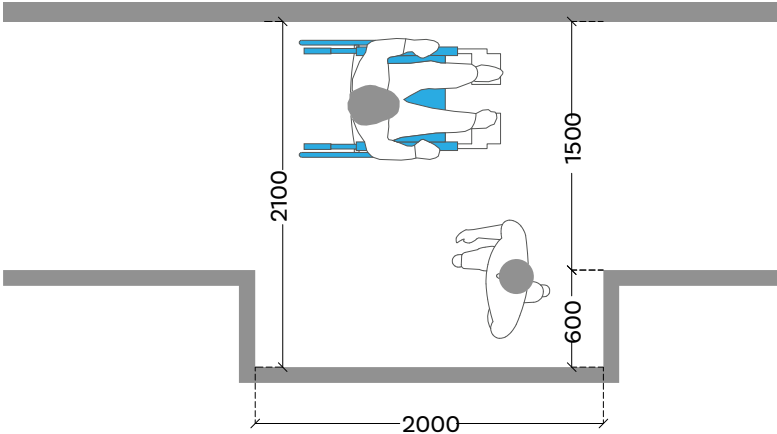
Figure 4.5 Dimension and space requirement for accessible corridor
